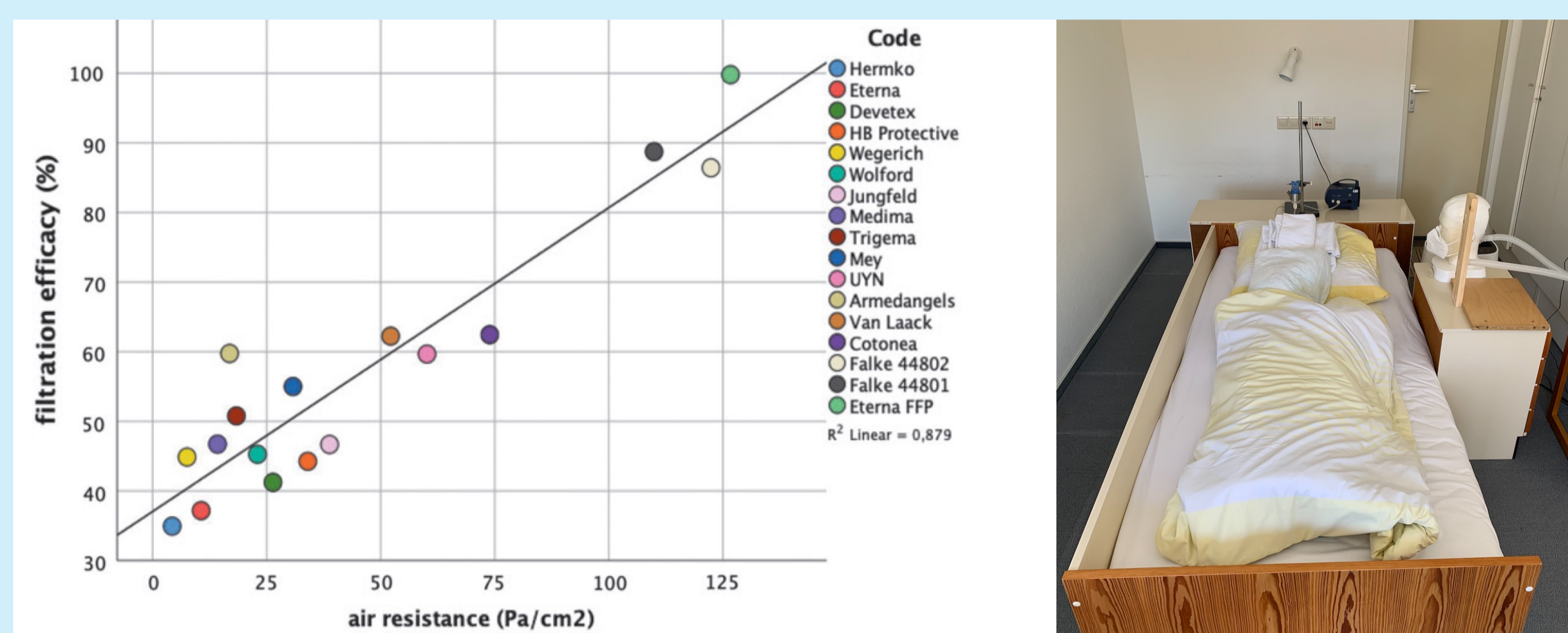
Filtration efficacy in % versus air resistance in Pascal/cm 2
